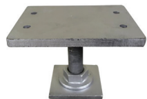
Straight 4 Holes 200mm L x 150mm W x 12mm WO-75-S4 // WO-90-S4 // WO-100-S4
