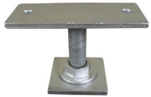
Straight 200mm L x 75mm W x 10mm WO-75-S // WO-90-S // WO-100-S
